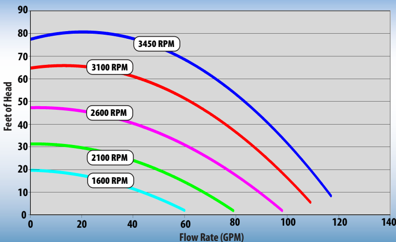
Econo Flo VSA-165 – Performance Curves
