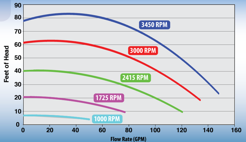
Econo Flo VSA Pump - Performance Curves
