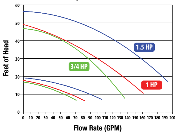
Hi-Flo II Pumps - Performance Curve
