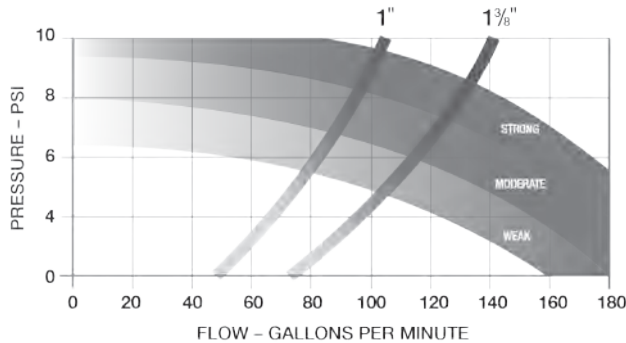
POWER STREAM JET FLOW CURVE
