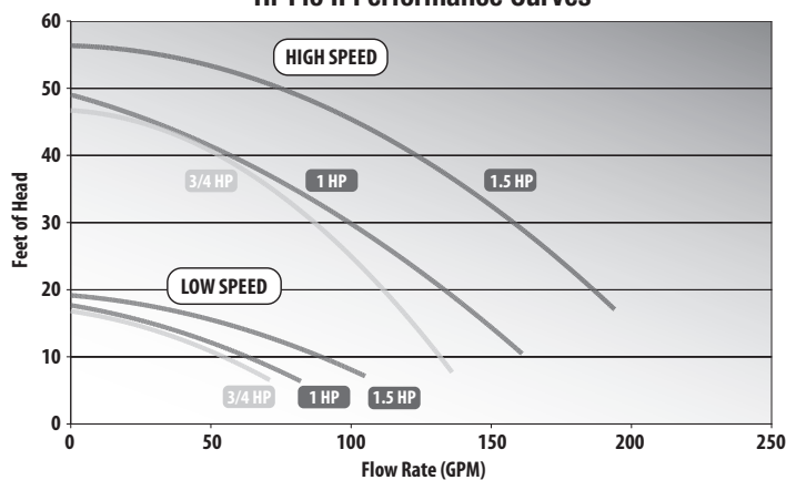
Hi-Flo II Performance Curves
