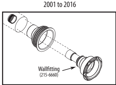
Power Gunite Storm Spa Jet Clip-in 215-6660 x = Color, 0 = White, 1 = Black, 7 = Gray
