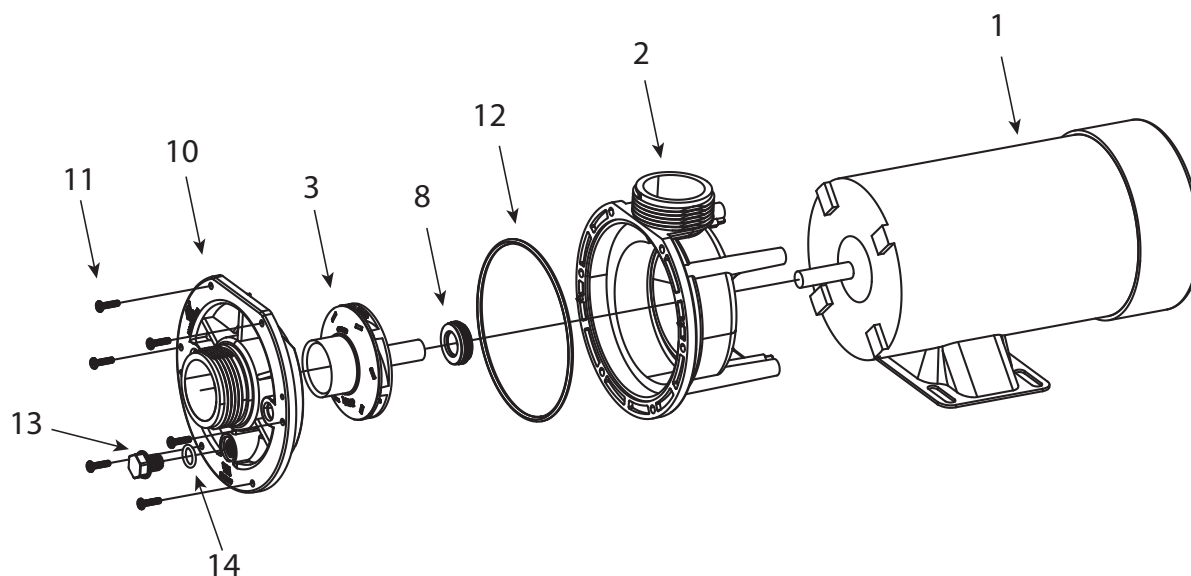
E-Series Center Discharge Pump Replacement Parts
