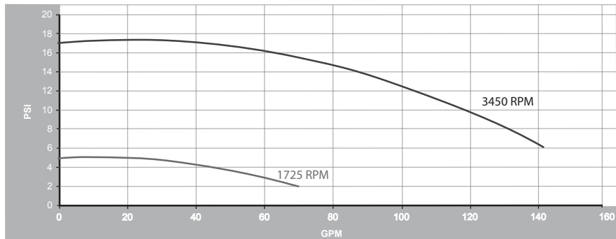
WATERWAY EX2, 9.5/3.2 A , 115V, 1.0 BHP
