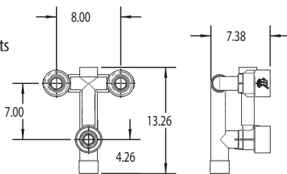
7" Gunite - 3-Jet Manifold
