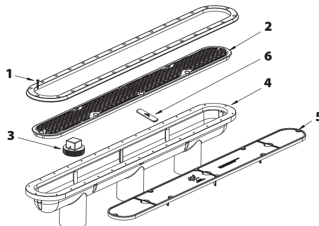
Vinyl Liner Strip Drain
