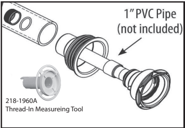
Power Gunite Storm Spa Jet Thread-In - Upgrade Kit - 400-6710 (Includes: Fitting, Threaded Ring w/ O-ring & Measuring Tool)
