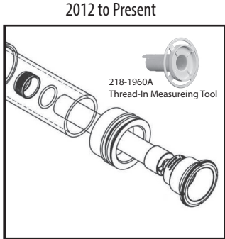
Poly Gunite Storm Spa Jet Thread-In - Upgrade Kit - 400-119x (Includes: Fitting, Threaded Ring w/ O-ring & Measuring Tool)
