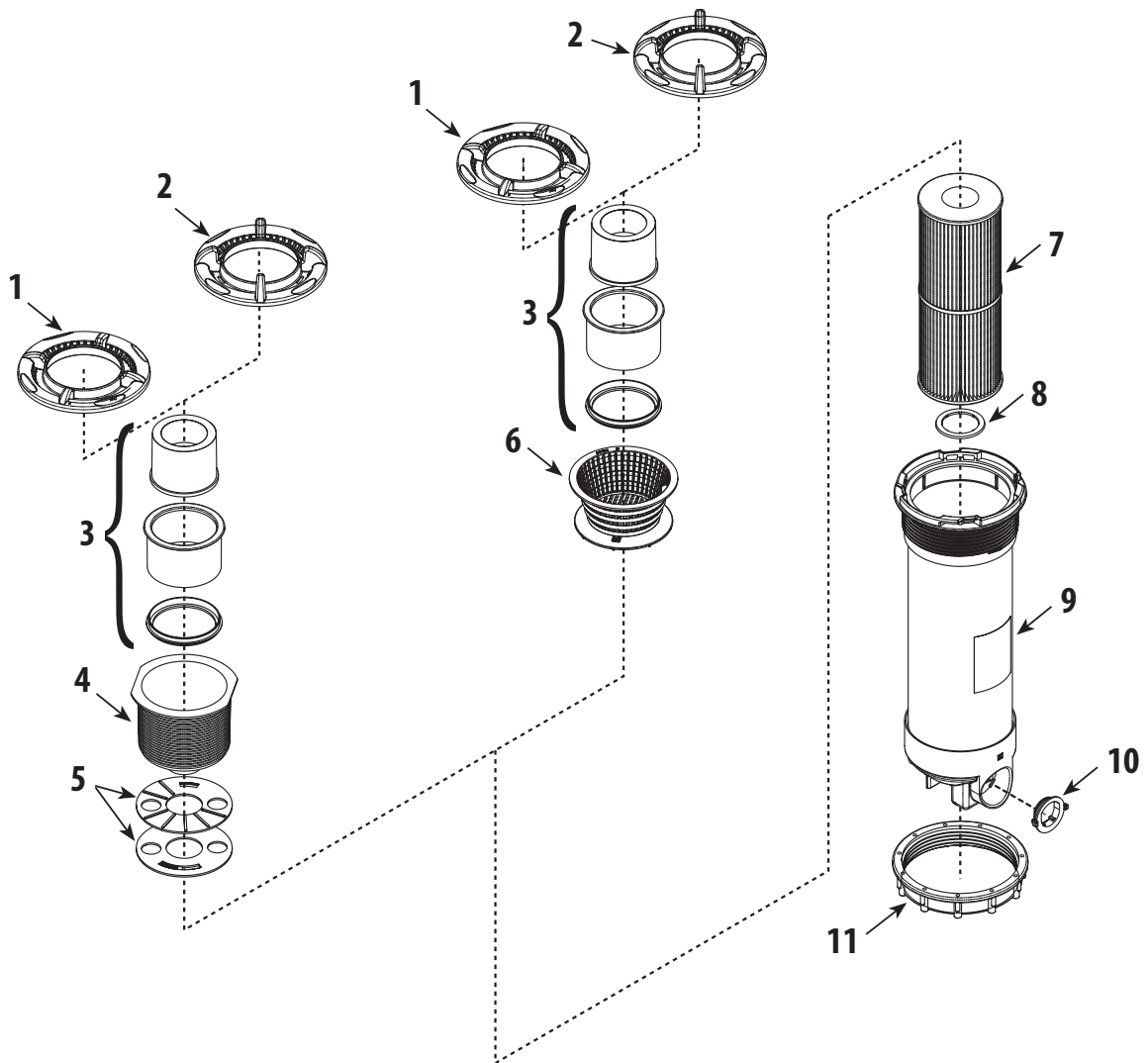
Dyna-Flo Top Mount Skim Filter Replacement Parts
