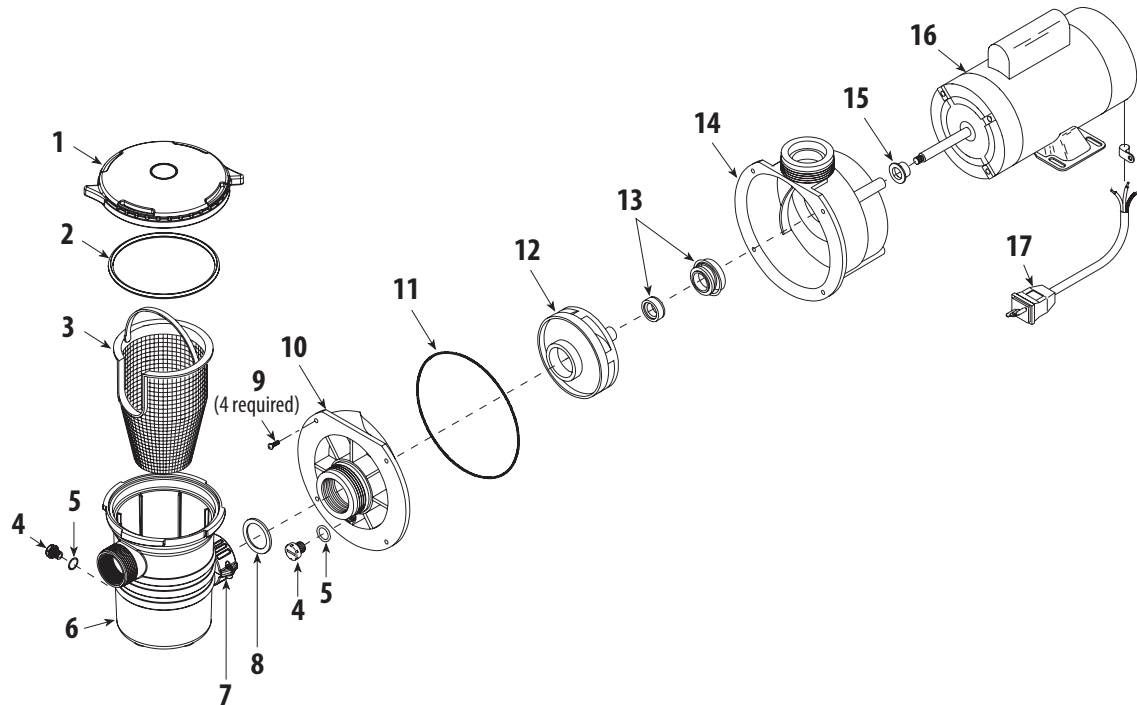
Center Discharge Pump Replacement Parts
