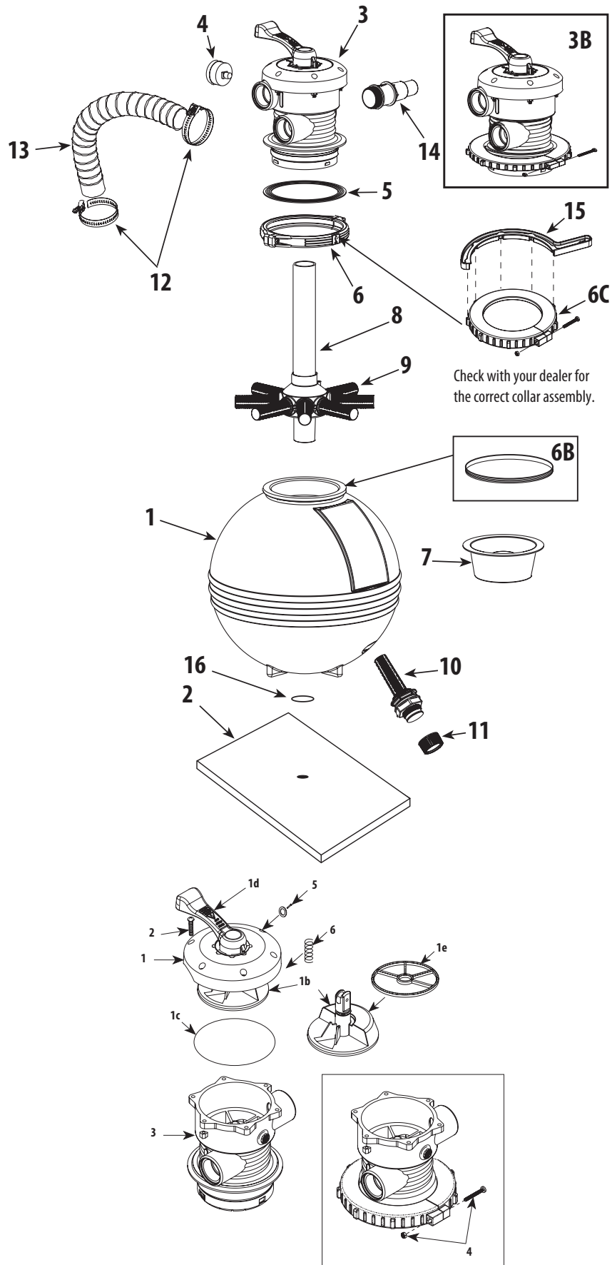
Multi-Port Valve Assembly
