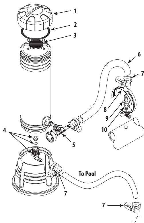
Off-Line Chlorinator
