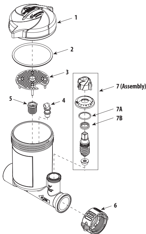
Above Ground In-Line Chlorinator
