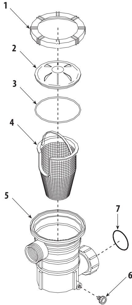
6" Trap (1999 and Earlier) Replacement Parts
