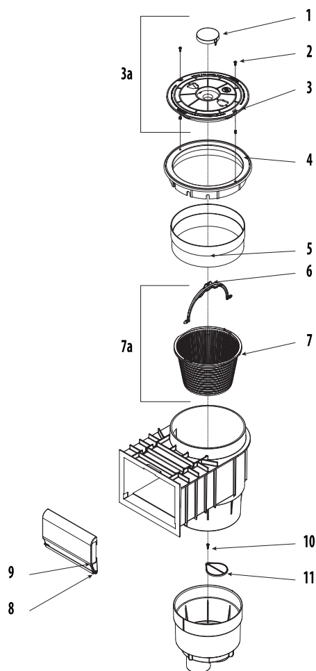
Renegade Gunite In-Ground Skimmer
