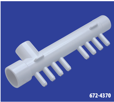
MANIFOLD TEE 1" SPG x 1" S x (8) \frac{3}{8} " SB
