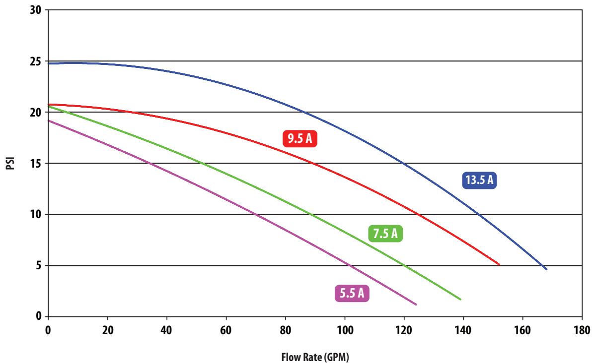
Genesis Generation Bath Pumps - Performance Curves
