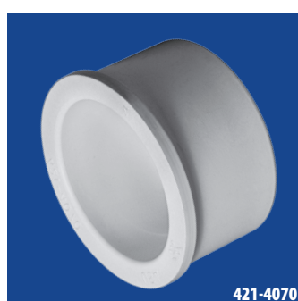
REDUCER 1 \frac{1}{2} " S x 2" SPG Part No. Bulk Qty. 421-4070 100
