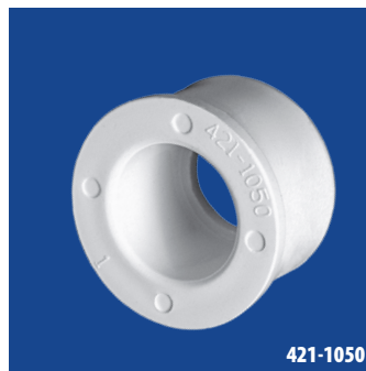
REDUCER 1" SPG x \frac{1}{2} " S Part No. Bulk Qty. 421-1050 225
